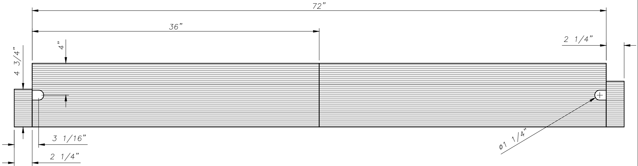
TYPE 3 X 8148 PREP FOR OPCON ON 72" PAIR OF DOORS CENTER HUNG TOP VIEW (REMOVABLE "B" SECTION, STRAIGHT EDGE)
