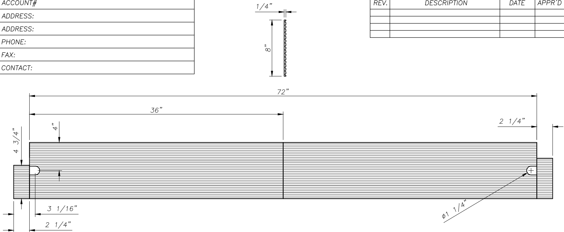
TYPE 4 X 8148 PREP FOR OPCON ON 72" PAIR OF DOORS CENTER HUNG TOP VIEW (REMOVABLE "B" SECTION, STRAIGHT EDGE)
