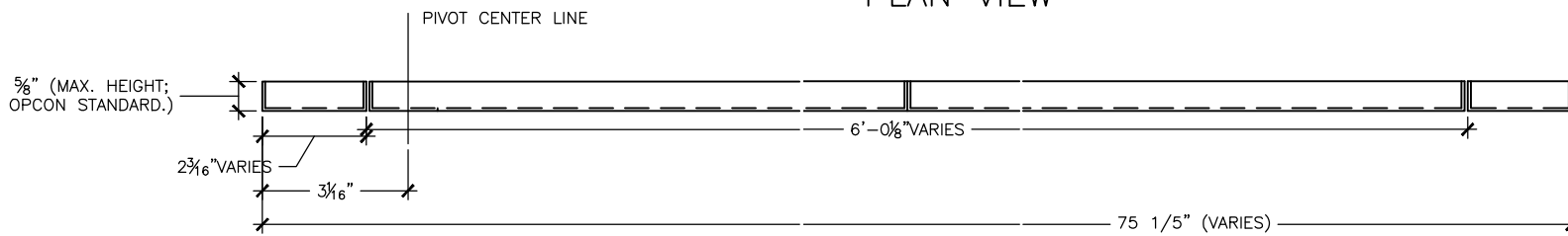
PLAN VIEW
