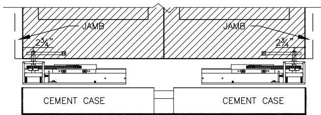
(CEMENT CASES SHOWN BELOW CONVERTER) CENTER HUNG DOORS - PAIR
