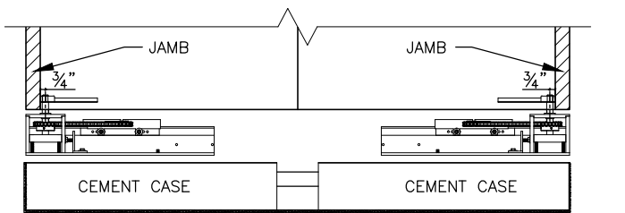
CONNECTING CONDUIT (CEMENT CASES SHOWN BELOW CONVERTER) OFFSET HUNG DOORS - PAIR CENTER LINE OF OPCON PIVOT MATCHES CENTERLINE OF DOOR PIVOT
